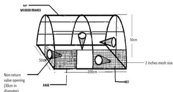
Figure 3: A sketch of a modified semi-circular Malian trap. Source: (Field design, 2018)
